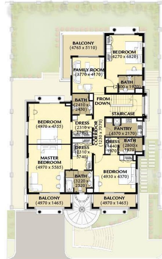
2nd Level (233 sqm) / Terrace (30 sqm)
